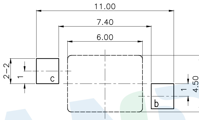
Hole Layout(top view)
