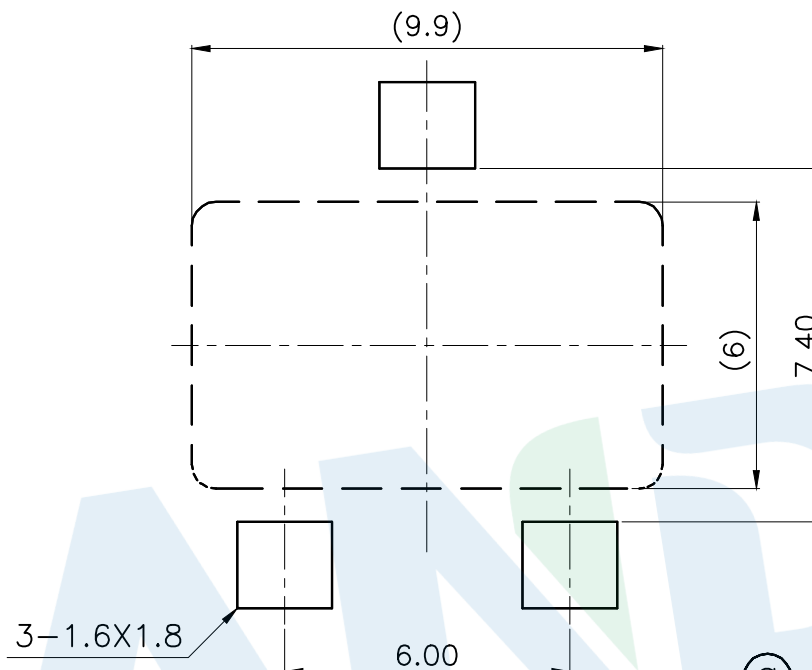
Hole Layout(top view)
