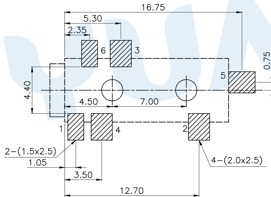
P.C.B LAYOUT(Copper-side view)
